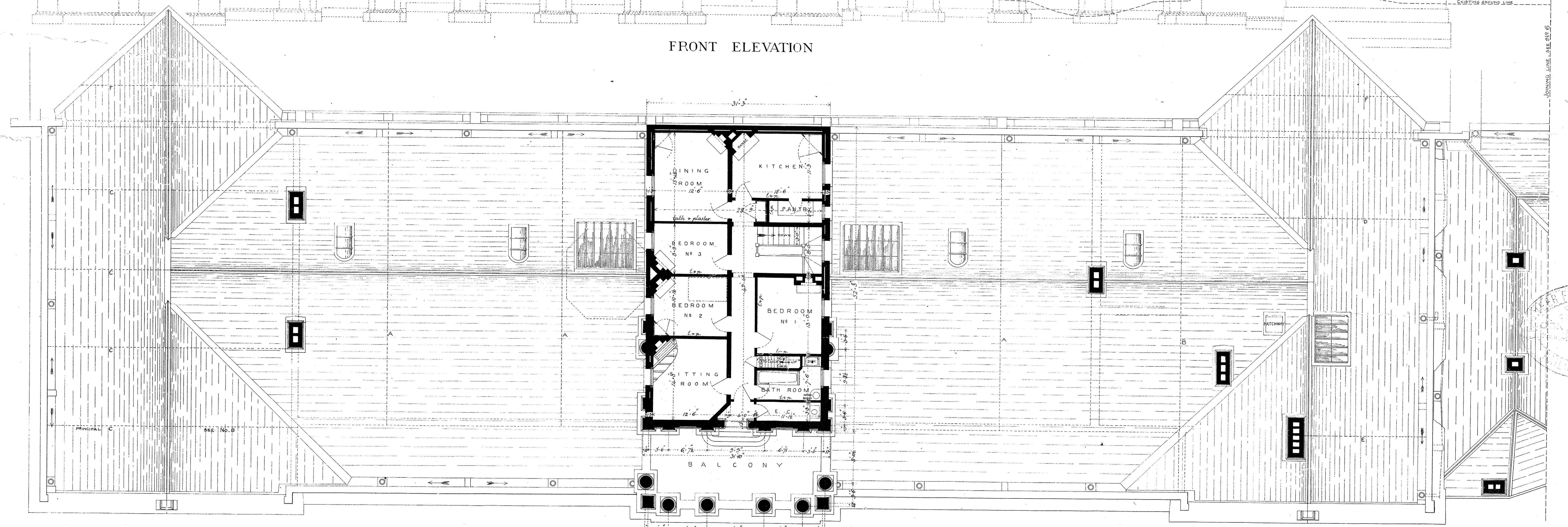
ROOF AND FIRST FLOOR PLAN
