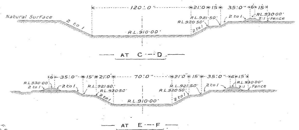
CROSS SECTIONS OF RESERVOIR
