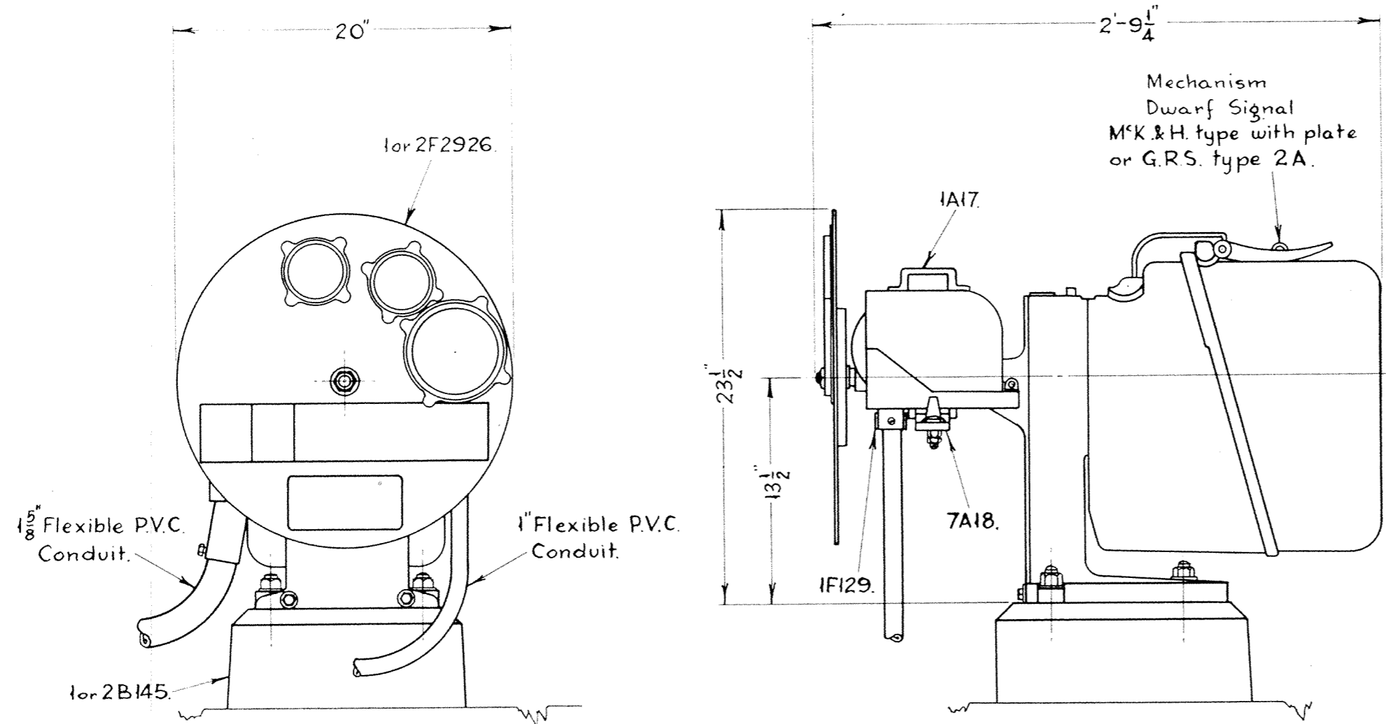
Dimensions for G.R.S. Mechanism.
